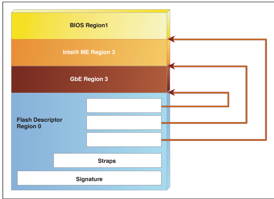
Figure 7.5 High Level Map of the Nonvolatile Memory
