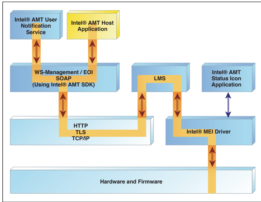
Figure 7.10 Local Software Components of Intel® AMT
