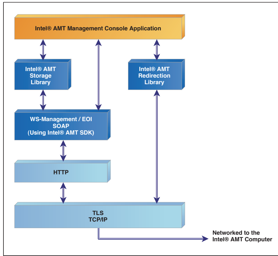
Figure 7.11 Remote Software Components of Intel® AMT
