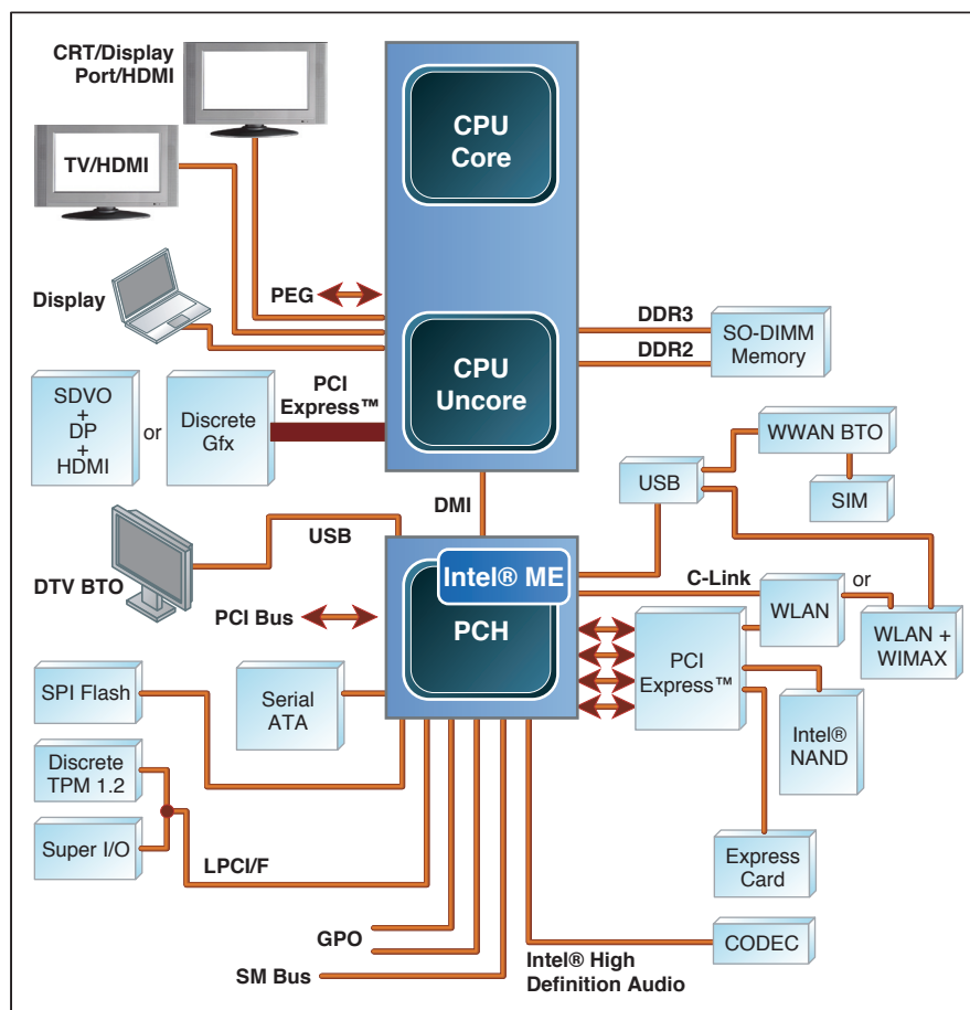
Figure 7.3 Hardware Architecture of Future Intel Platforms
