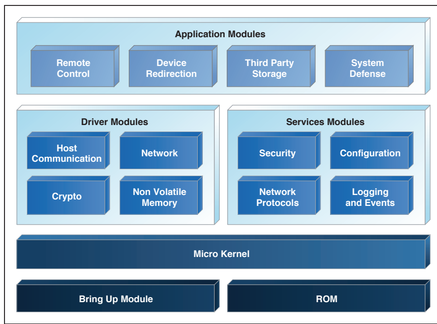
Figure 7.7 Intel® Management Engine Firmware Block Diagram
