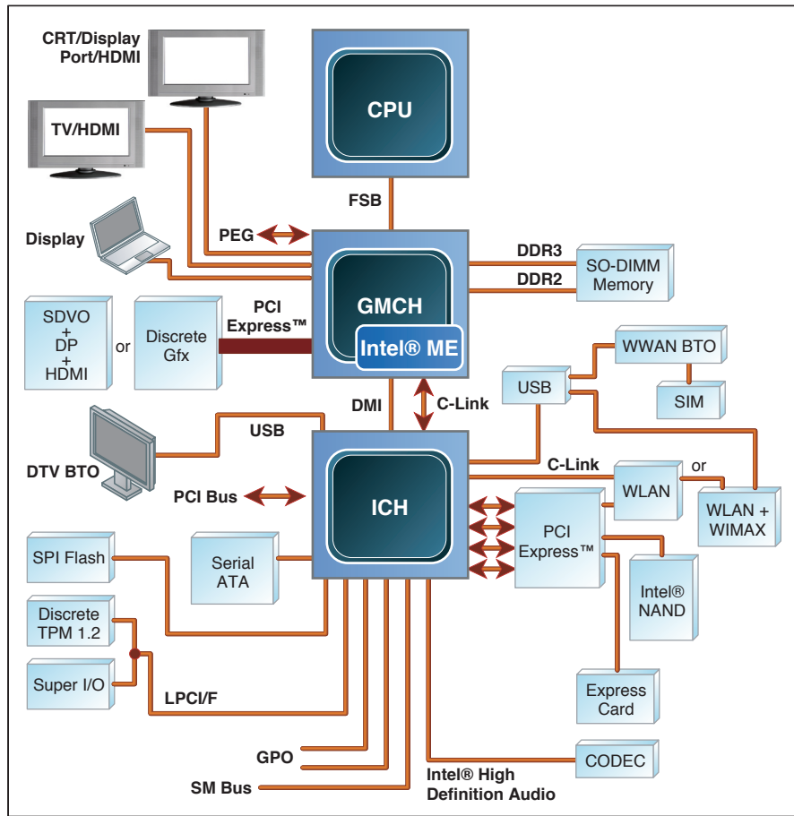
Figure 7.2 Hardware Architecture of an Intel Platform
