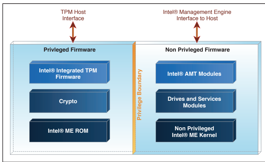
Figure 7.8 Intel® ME Kernel: Privileged and Non-Privileged Partitions
