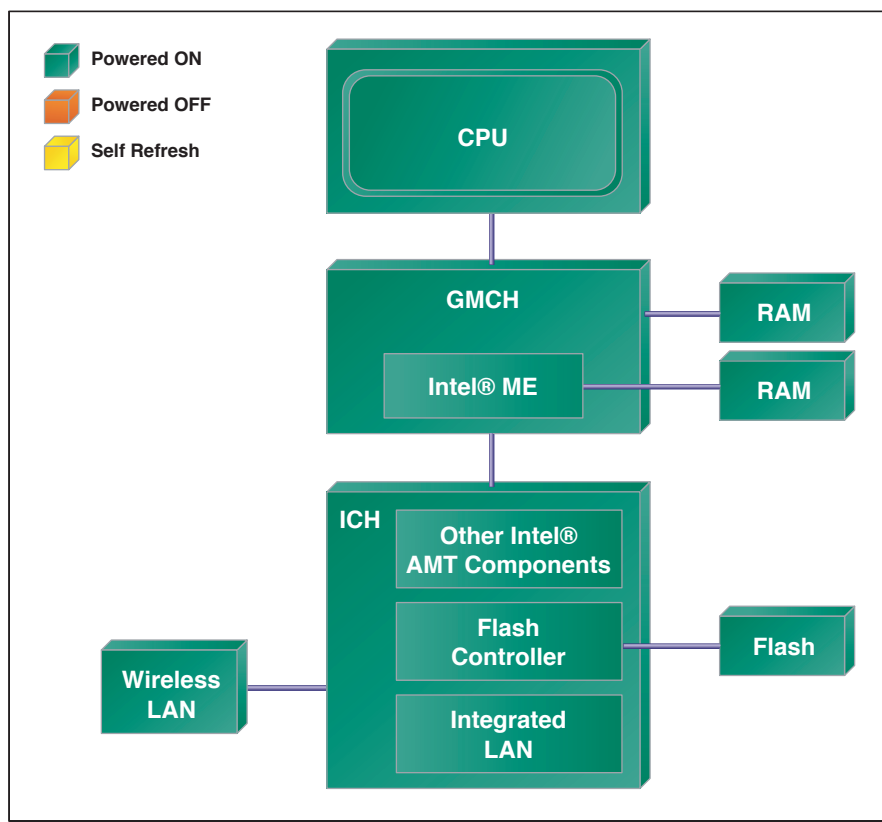
Figure 7.13 An Intel® AMT Computer in S0 and M0 State
