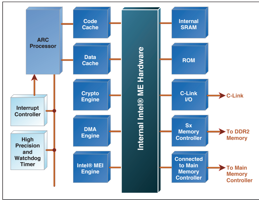
Figure 7.4 Hardware Architecture of the Intel® Manageability Engine
