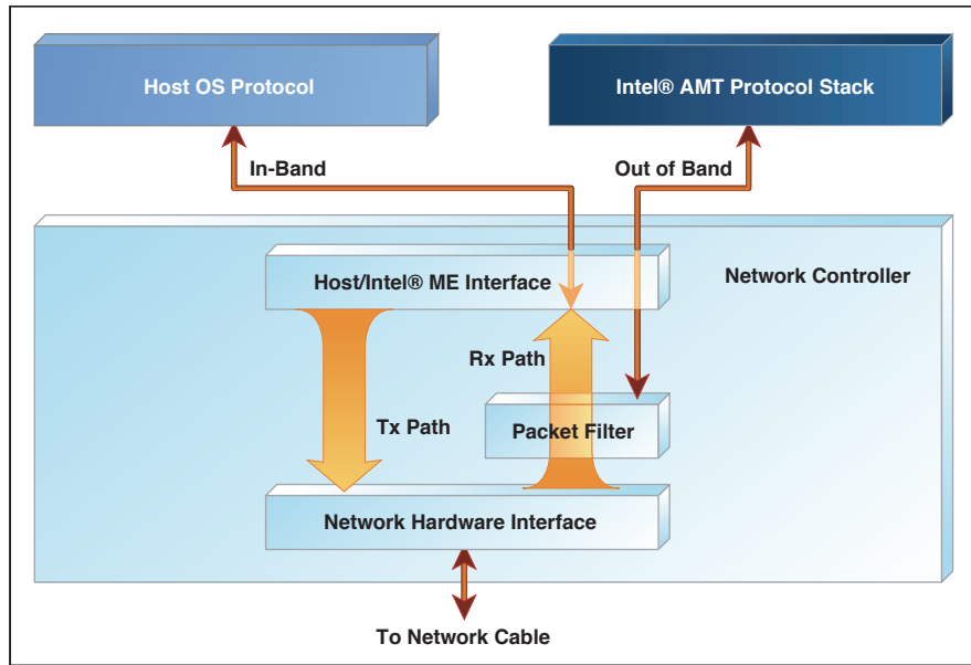
Figure 7.6 Network OOB Filters for Gigabit Ethernet
