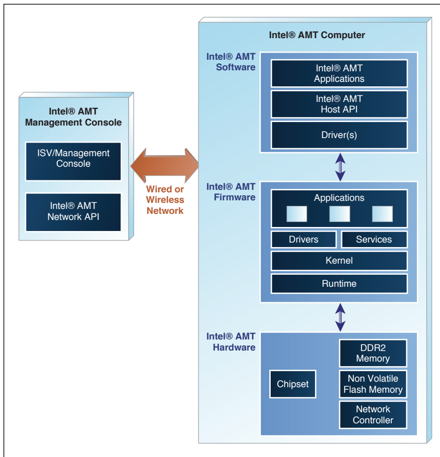
Figure 7.1 High Level View of Intel® AMT components
