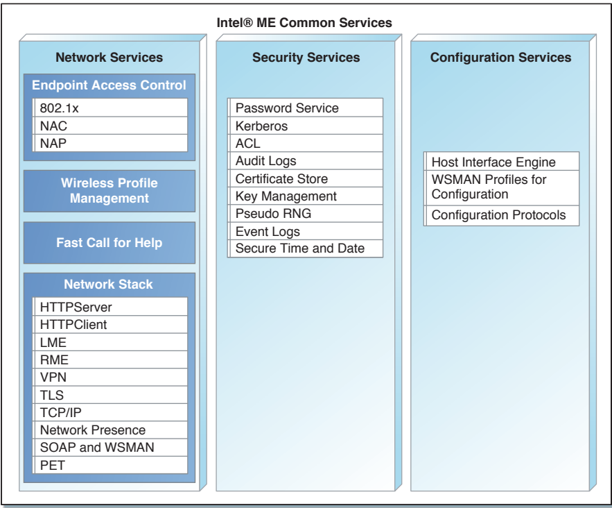
Figure 7.9 Intel® ME Common Services
