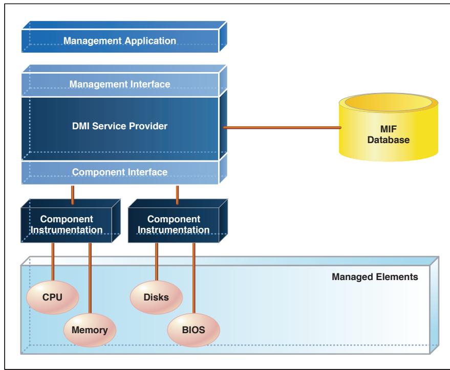
Figure 2.3 DMI Service Provider Infrastructure
