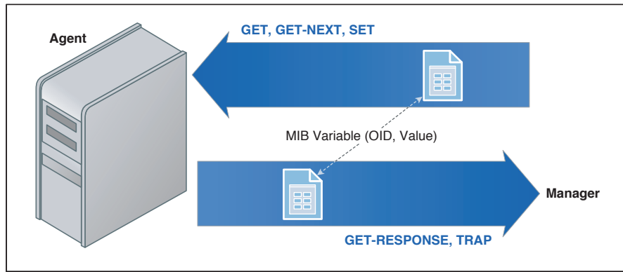
Figure 2.2 SNMP Protocol Messages
